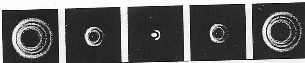
Fig 7-2 Even though the star pattern appears the same on both sides of focus, they are asymmetric. The dark obstruction is skewed off to the left side of the diffraction pattern indicating poor collimation.
