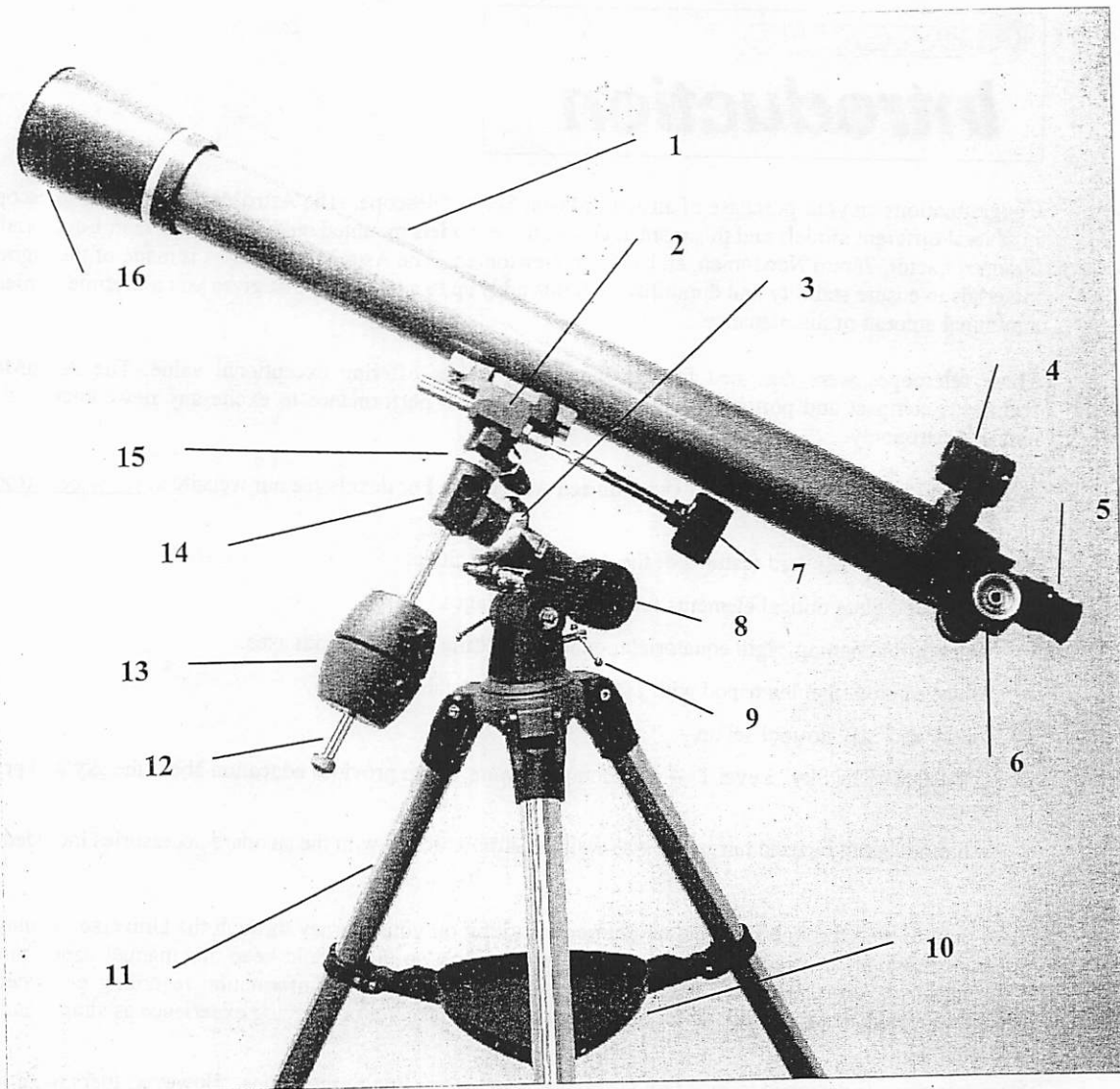
Figure 1-1 AstroMaster 70 EQ Refractor
