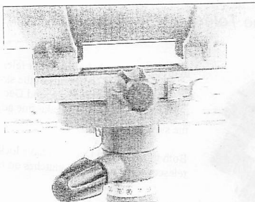
Figure 2-18 Mounting Knob & Safety Screw in the dovetail bracket Shown is the 114EQ telescope tube
